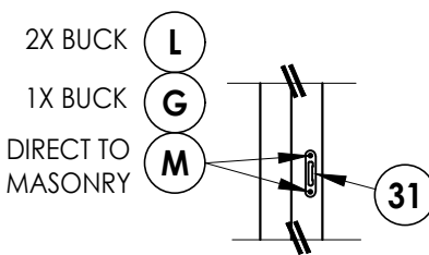
TONGUE STRIKE DETAIL
