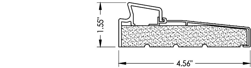
33 INSWING THRESHOLD Inswing Basic Fixed Sill
